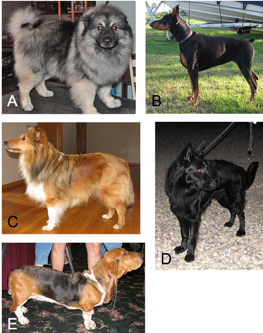
Figure 1. Coat color variation attributed to the ASIP locus. (A) a wolf sable ( a^w ) Keeshond, (B) a black-and-tan ( a^t ) Doberman Pinscher, (C) a fawn ( a^f ) Shetland Sheepdog, (D) a recessive black ( a ) German Shepherd Dog, and (E) a saddle tan Basset Hound.
