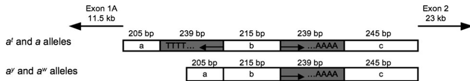
Figure 2. An illustration of an 1143-bp fragment, from 5' of the ASIP start codon in exon 2, obtained from genomic DNA from a black-and-tan ( a' ) Shetland Sheepdog and a wolf sable ( a'' ) Siberian Husky. Shaded boxes represent SINEs, with arrows denoting orientation. Segments a, b, and c of this fragment are present in all dogs.
